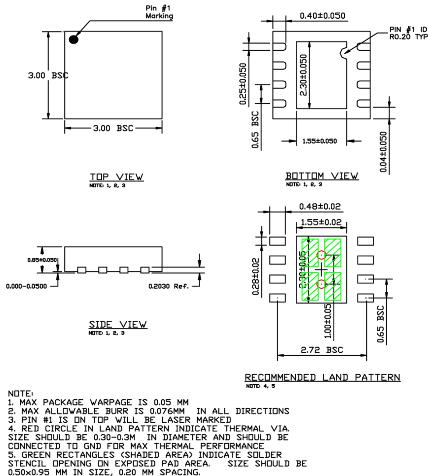
8-Pin 3mm × 3mm DFN (ML)
