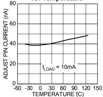
MIC29512 Adjust Pin Current vs. Temperature
