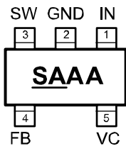
5-Pin SOT23 (YM5)
