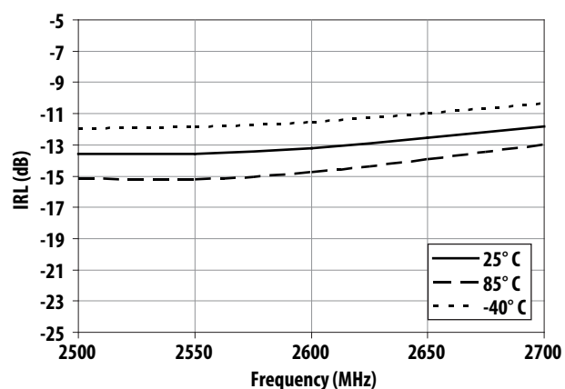
Figure 20. Over Temperature IRL vs Frequency
