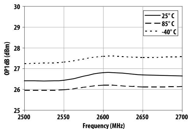
Figure 18. Over Temperature OP1dB vs Frequency
