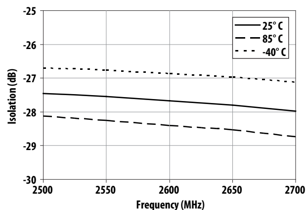
Figure 22. Over Temperature Isolation vs Frequency
