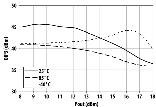
Figure 14. Over Temperature OIP3 vs Pout at 1900 MHz
