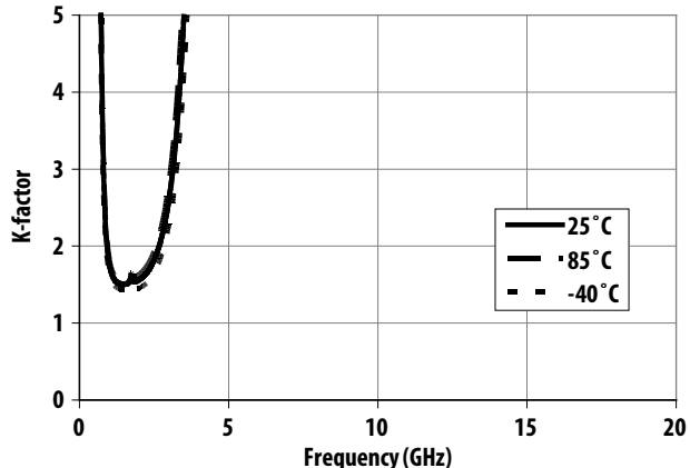
Figure 16. Over Temperature K-factor vs Frequency
