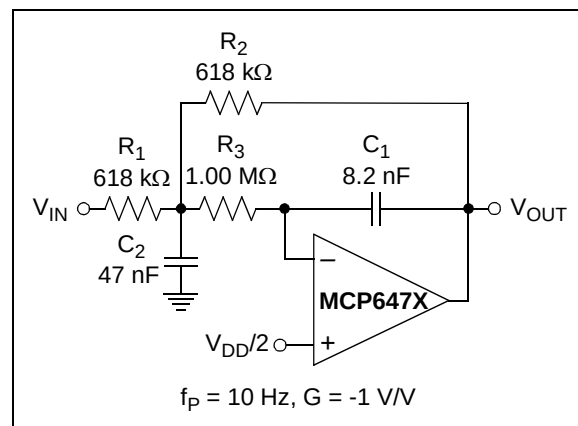
FIGURE 4-11: Second-Order, Low-Pass Butterworth Filter with Multiple-Feedback Topology.
