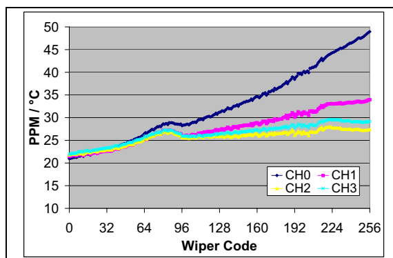
FIGURE 2-31: 10 kΩ – R_{WB} PPM/°C vs. Wiper Setting. ( R_{BW(\text{code}=n, 125^\circ\text{C})} - R_{BW(\text{code}=n, -40^\circ\text{C})} / R_{BW(\text{code}=256, 25^\circ\text{C})} / 165^\circ\text{C} * 1,000,000 ) ( V_{DD} = 5.5\text{V} , I_W = 150\text{ }\mu\text{A} ).
