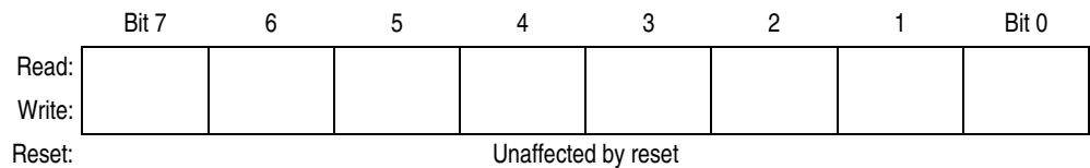
Figure 10-2. Accumulator (A)
