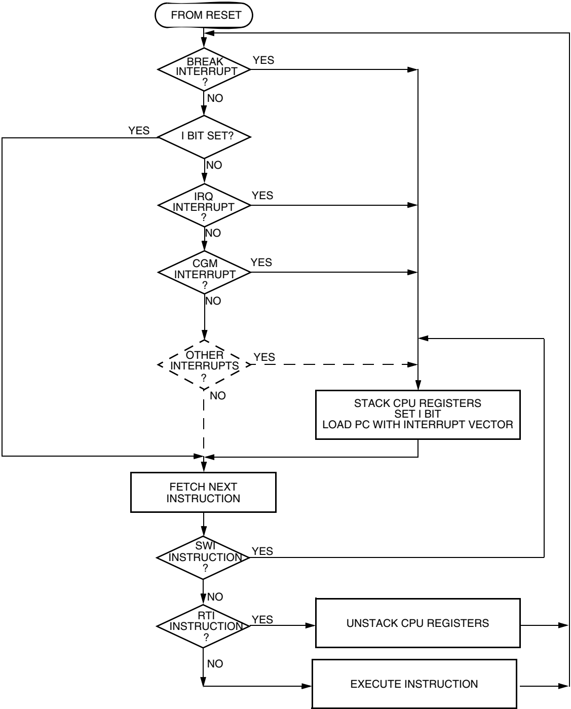
Figure 4-5. Interrupt Processing
