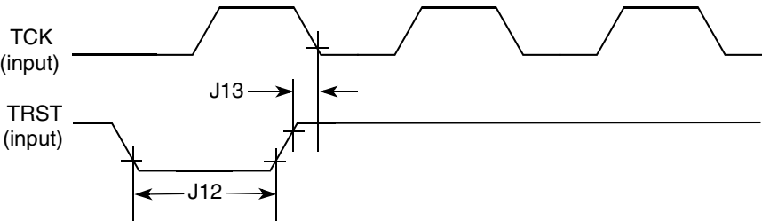
Figure 25. TRST Timing Diagram
