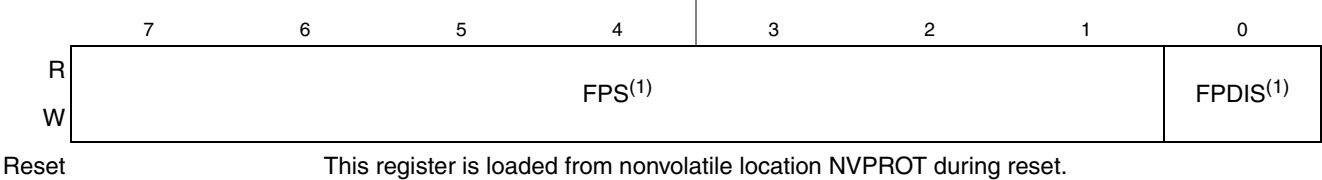
Figure 4-8. Flash Protection Register (FPROT)
