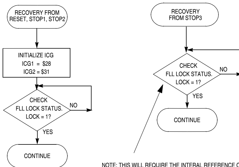
Figure 7-10. ICG Initialization and Stop Recovery for Example #3
