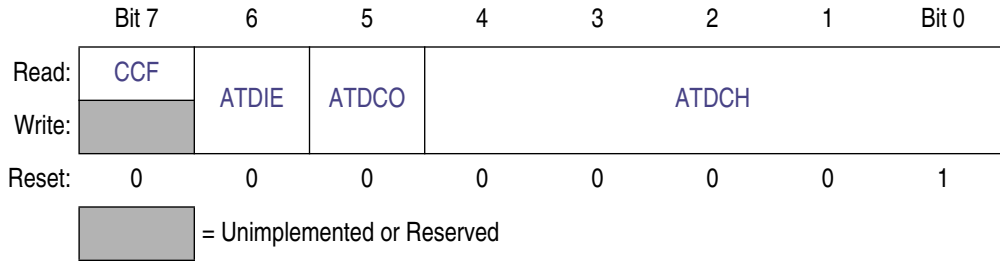
Figure 14-8. ATD Status and Control Register (ATD1SC)
