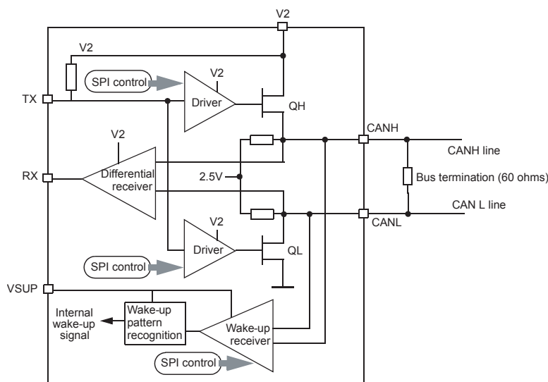
Figure 34. 33989 CAN Interface
