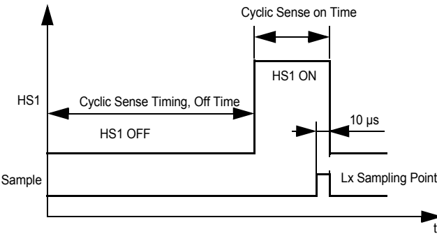
Figure 19. HS1 Operation when Cyclic Sense is Selected
