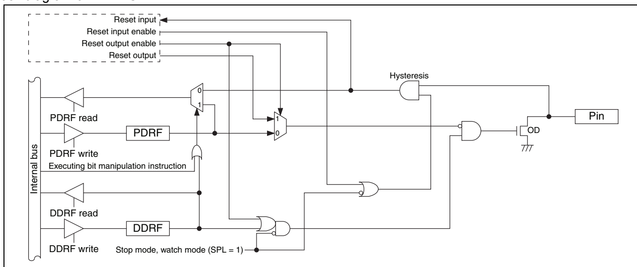
• Block diagram of PF2/ \overline{\text{RST}}
