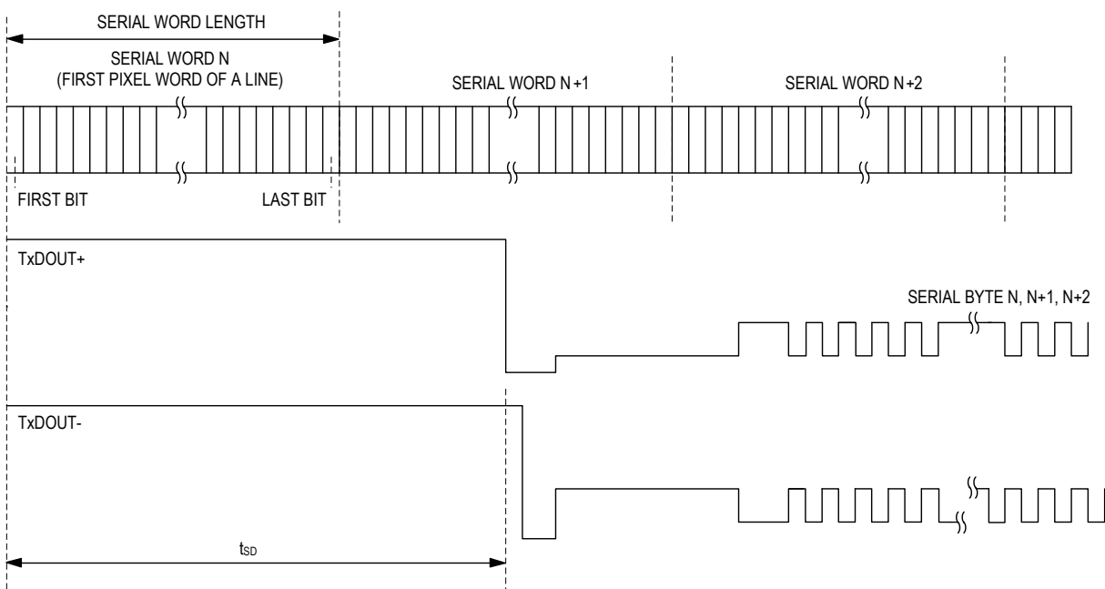
Figure 8. Deserializer Delay
