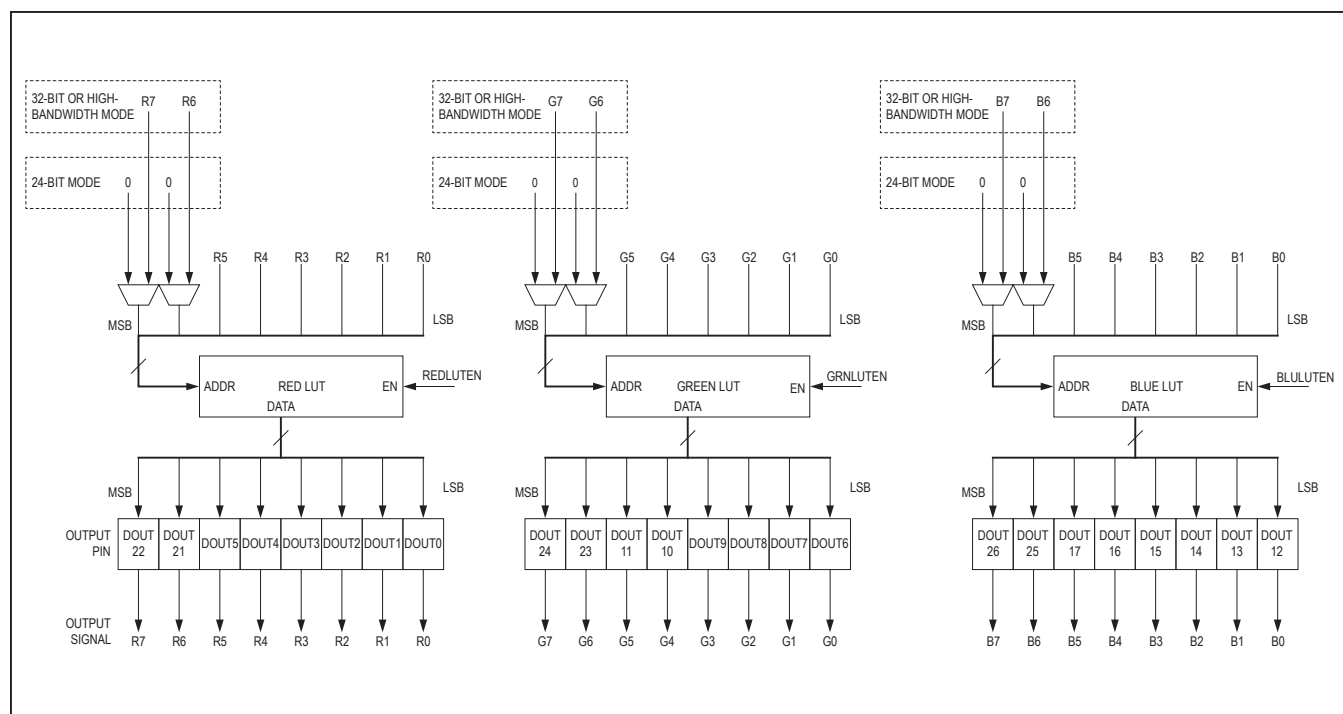
Figure 56. LUT Dataflow
