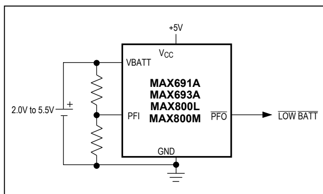
Figure 7. Low-Battery Indicator
