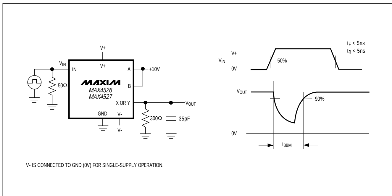
Figure 4. Break-Before-Make Interval
