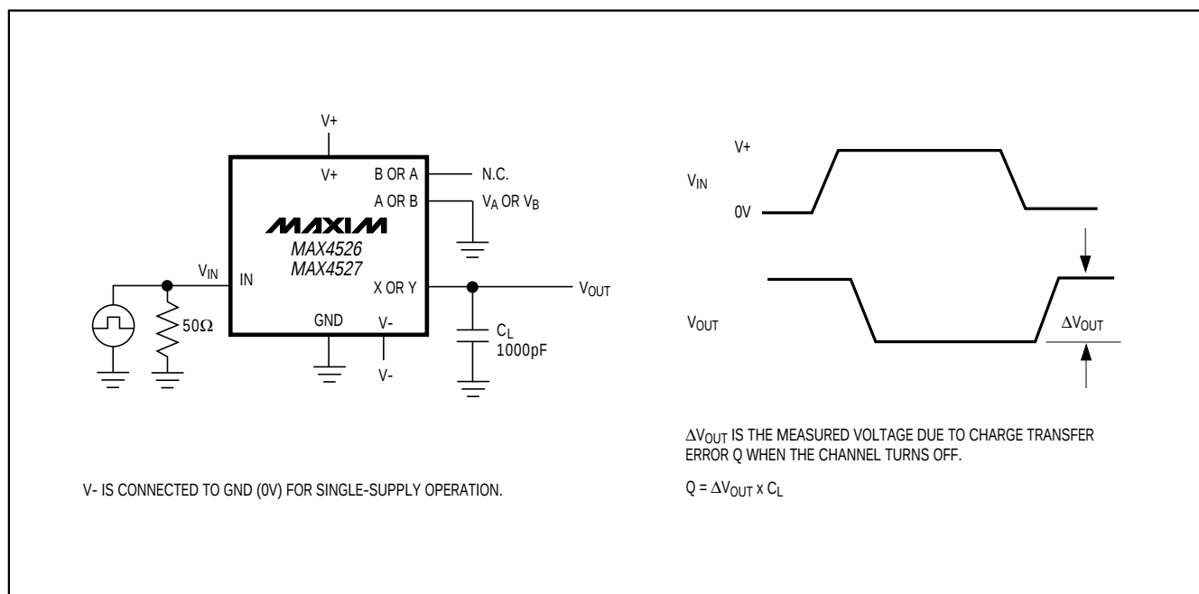
Figure 5. Charge Injection
