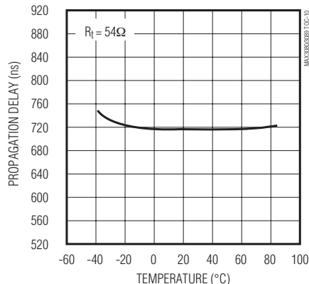
DRIVER PROPAGATION DELAY (500kbps MODE) vs. TEMPERATURE
