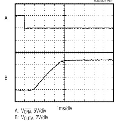
SWITCH TURN-ON TIME (MAX1823/MAX1823A)
