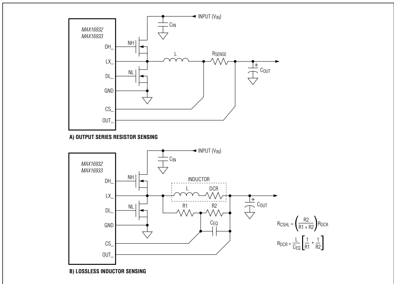
Figure 1. Current-Sense Configurations
