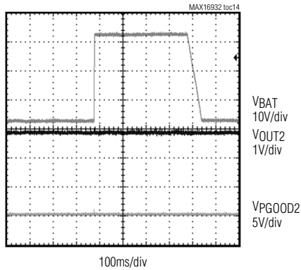
LOAD DUMP
