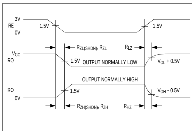
Figure 12. Receiver Enable and Disable Times (MAX1481/MAX1484 only)
