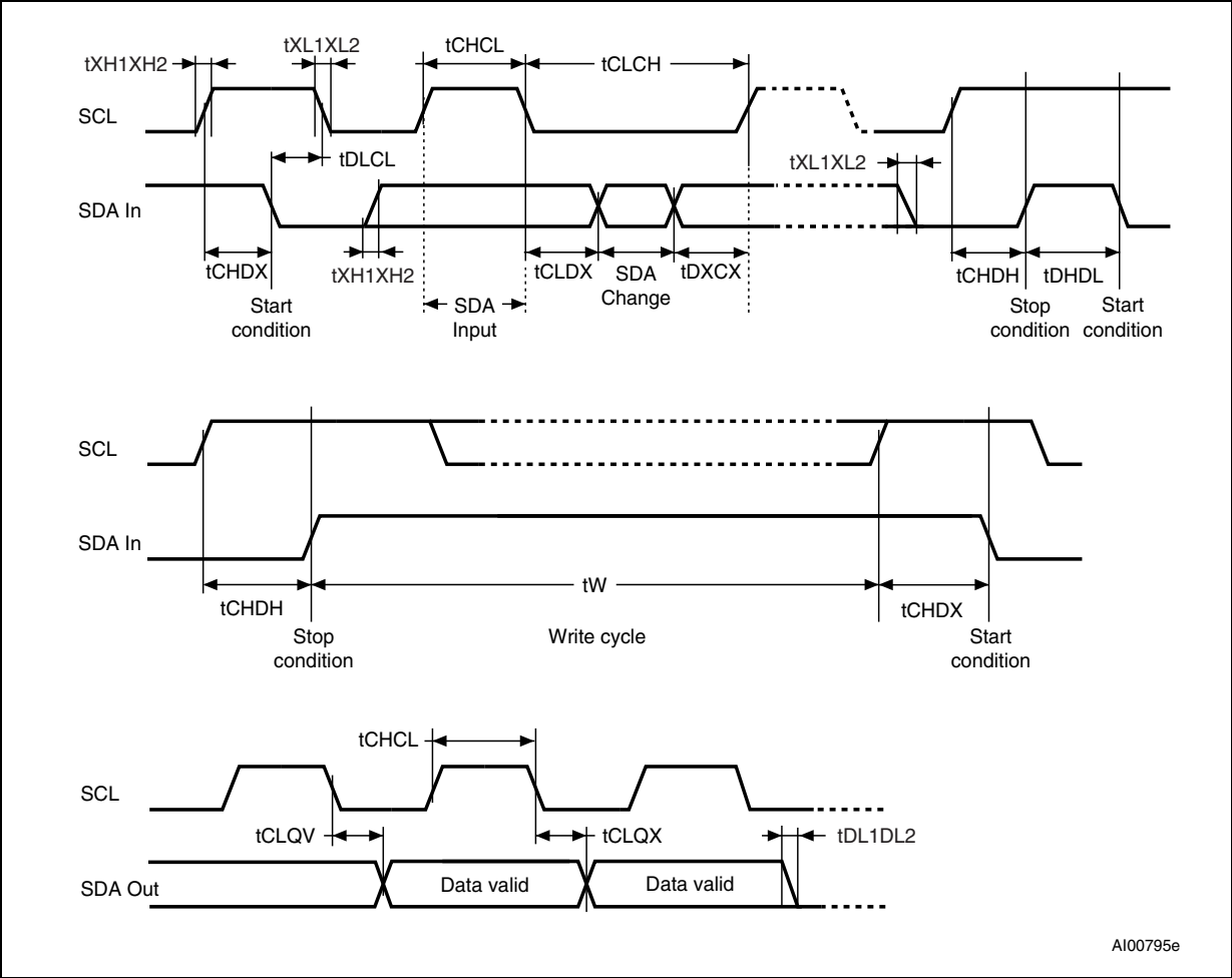
Figure 13. AC waveforms
