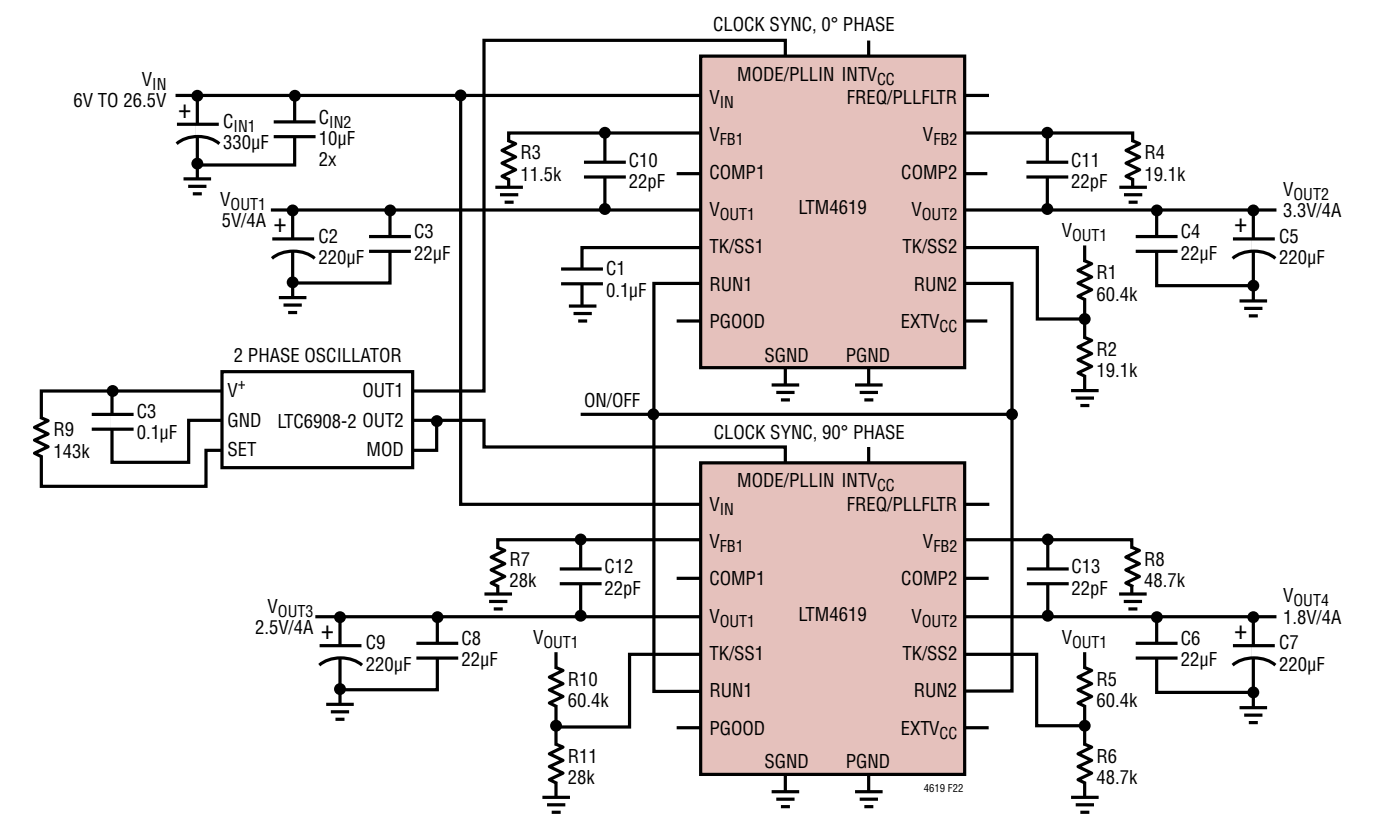
Figure 22. 4-Phase, Four Outputs (5V, 3.3V, 2.5V and 1.8V) with Tracking
