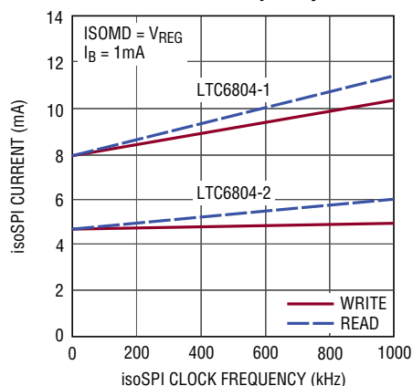
isoSPI Current (READY/ACTIVE) vs isoSPI Clock Frequency
