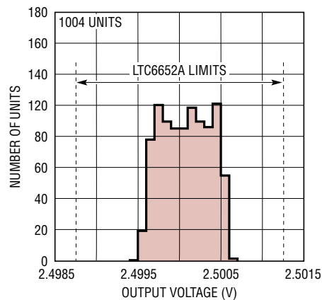
Typical V_{OUT} Distribution for LTC6652-2.5
