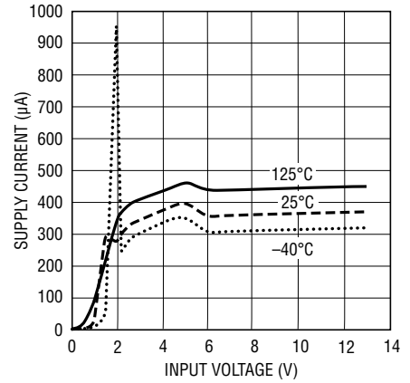
5V Supply Current vs Input Voltage
