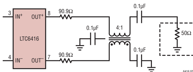
Figure 4. Output Termination for Differential 400Ω Load Impedance Using a 4:1 Balun
