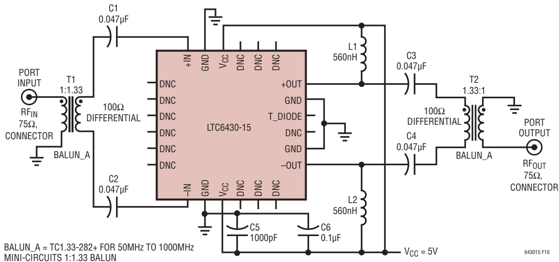
Figure 10. CATV Amplifier: 75 \Omega Input and 75 \Omega Output
