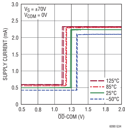
Supply Current vs \overline{\text{OD}} Pin Voltage
