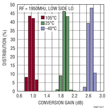
1950MHz Conversion Gain Distribution
