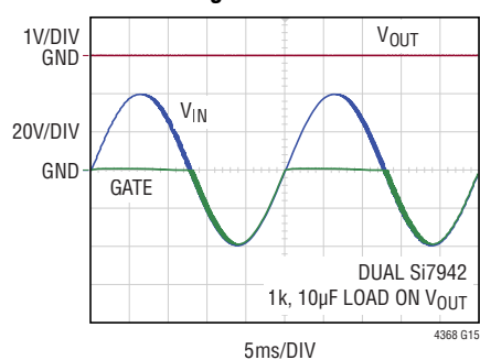
AC Blocking
