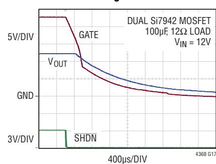
Turn-Off Timing
