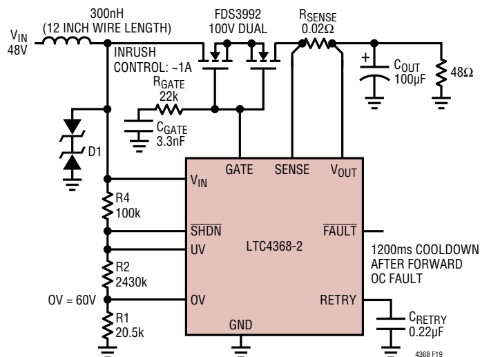
Figure 19. 0V Fault with Large V_{IN} Inductance
