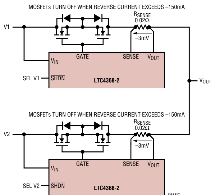
Figure 17. Alternative to Ideal Diode
