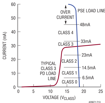
Figure 13. PD Classification
