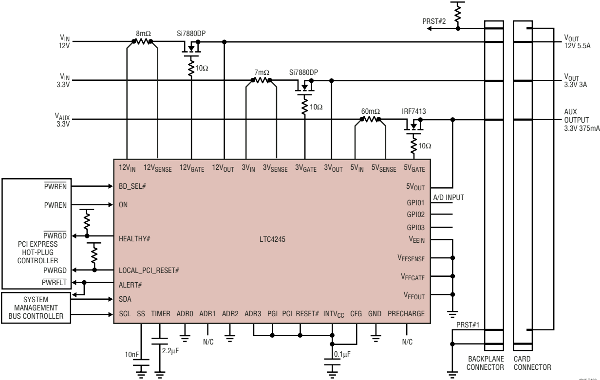
PCI Express Backplane Resident Application
