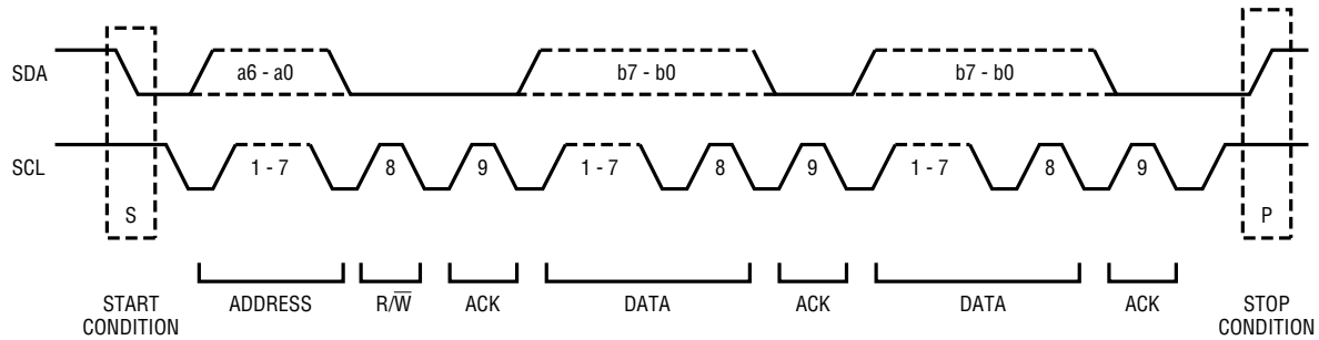
Figure 11. Data Transfer over I²C or SMBus
