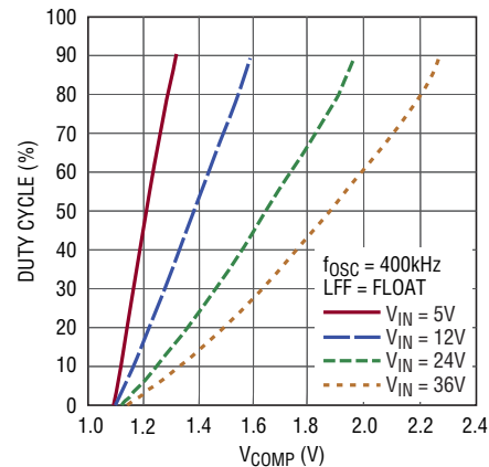
Duty Cycle vs V_{COMP} with Line Feedforward
