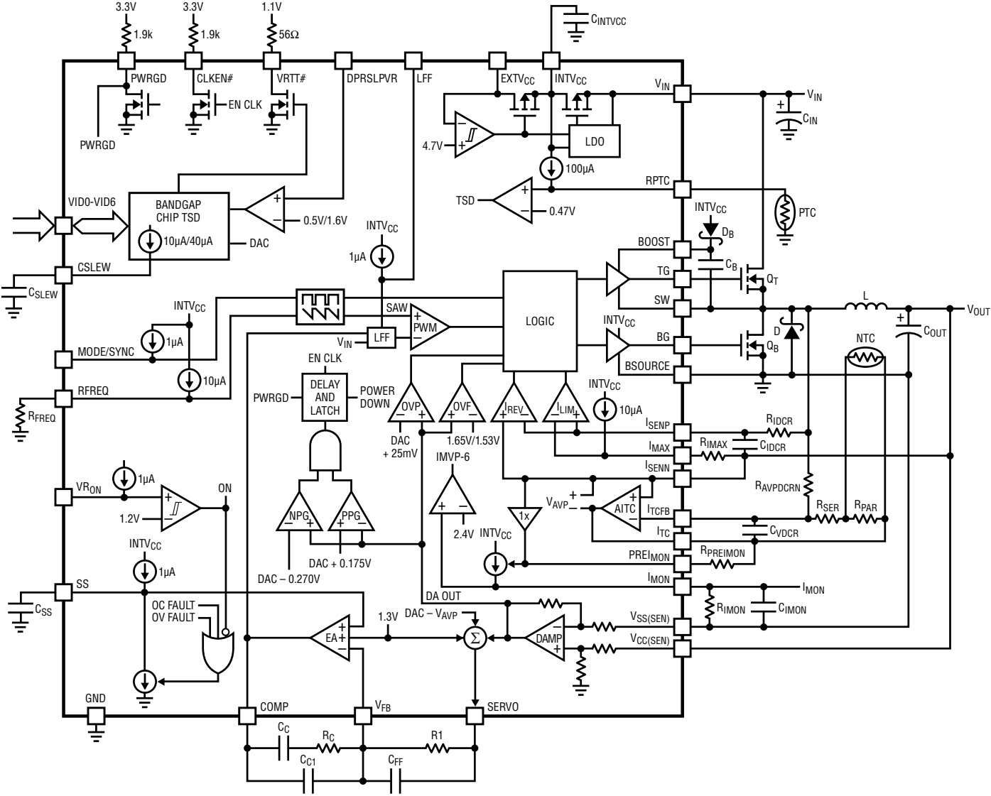
Figure 1. Functional Diagram
