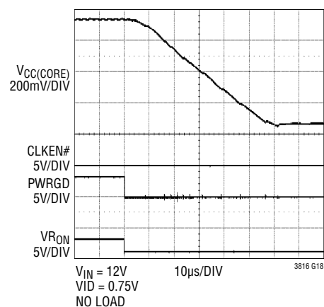
VR_{ON} Shutdown
