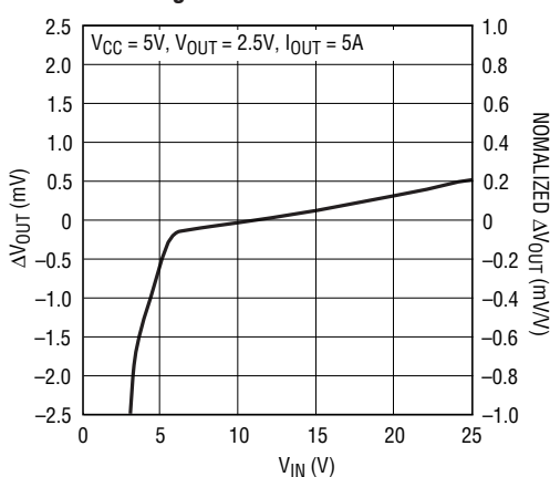
Line Regulation
