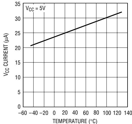
V_{CC} Shutdown Current vs Temperature
