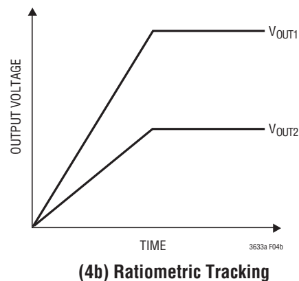
Figure 4. Two Different Modes of Output Voltage Tracking
