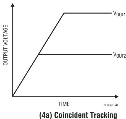
Figure 4. Two Different Modes of Output Voltage Tracking
