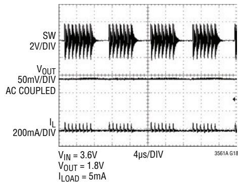
Switching Waveforms
