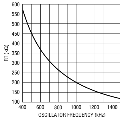
Oscillator Programming Resistor
