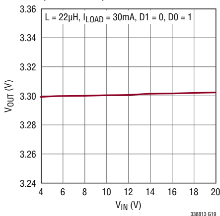
V OUT Line Regulation (LTC3388-3)
