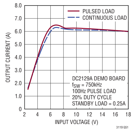
Maximum Output Current V_{OUT} = 5V
