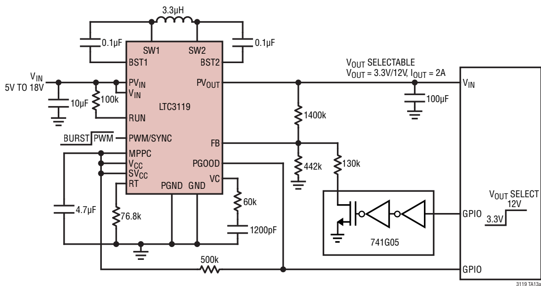
Selectable 12V or 3.3V Output, 1MHz Regulator
