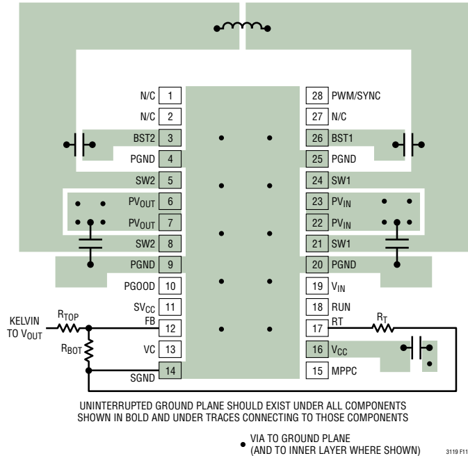
Figure 11. PCB Layout Recommended for the FE Package
