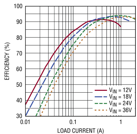
PWM Mode Efficiency, V_{OUT} = 24\text{V} , f_{SW} = 1\text{MHz}
