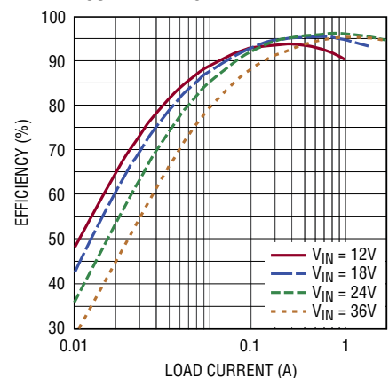
PWM Mode Efficiency, V_{OUT} = 24\text{V} , f_{SW} = 500\text{kHz}
