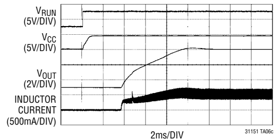
Soft-Start Waveform, V_{IN} = 24V , I_{LOAD} = 0.5A
