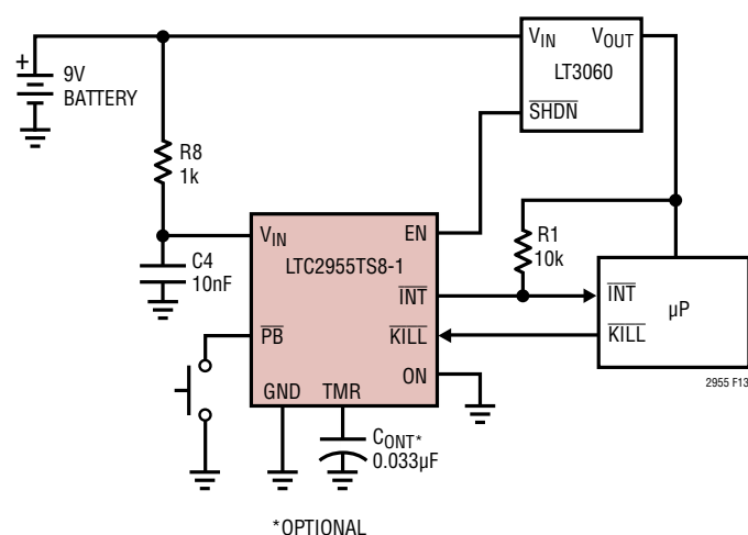
Figure 13. Enhancing V_{IN} Ruggedness
