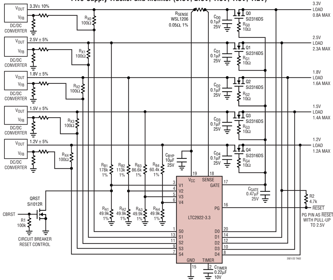
Five-Supply Tracker and Monitor (3.3V, 2.5V, 1.8V, 1.5V, 1.2V)
