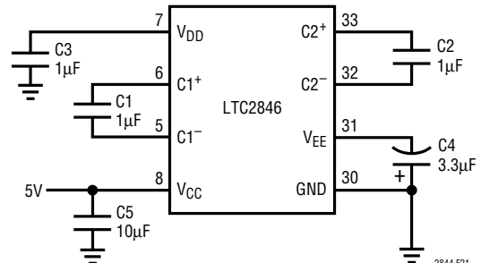
Figure 21. Charge Pump
