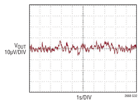
Output 0.1Hz to 10Hz Voltage Noise
