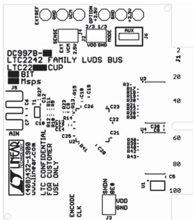
Silkscreen Top
