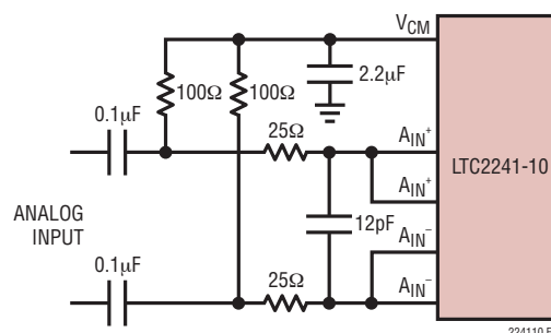
Figure 5. Capacitively-Coupled Drive
