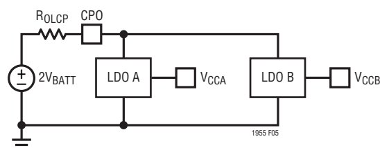
Figure 5. Equivalent Open-Loop Circuit
