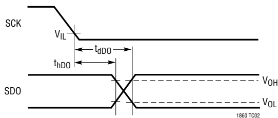
Voltage Waveforms for SDO Delay Times, t_{dDQ} and t_{hDQ}
