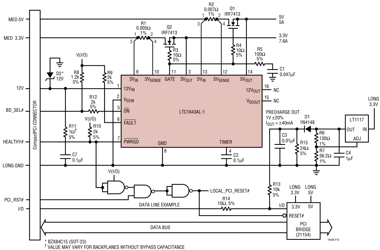
Figure 10. CompactPCI Application without ±12V Outputs
