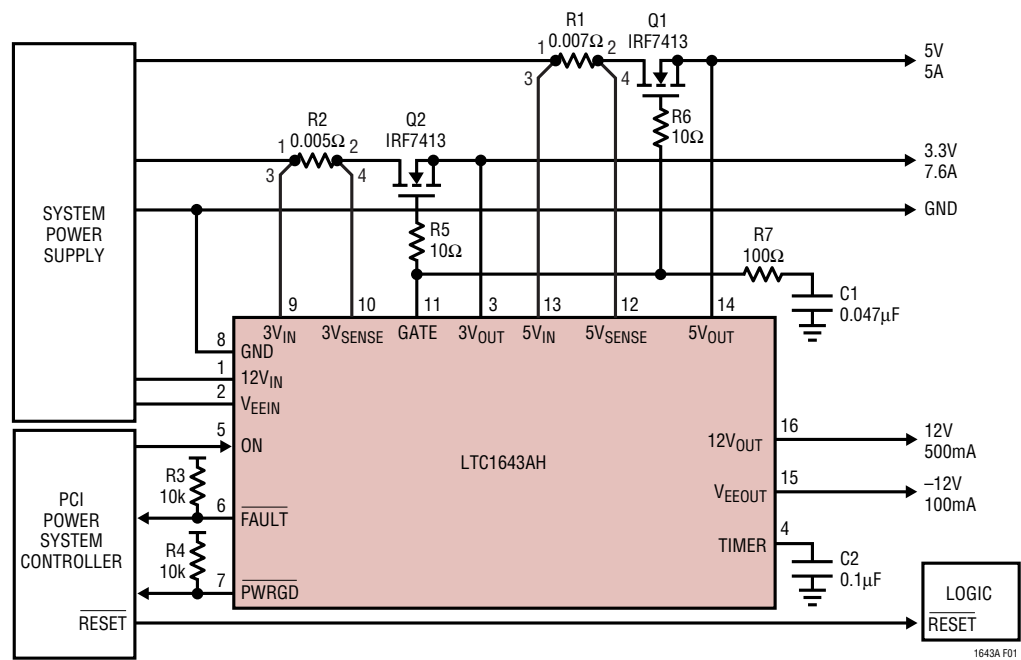
Figure 1. Typical PCI Application
