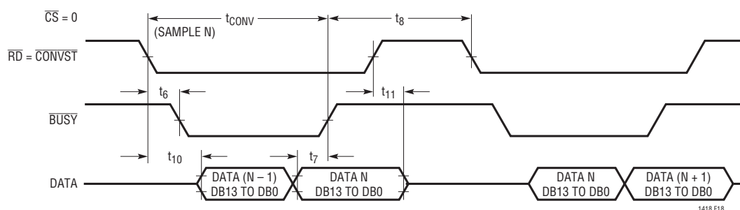
Figure 18. Slow Memory Mode Timing
