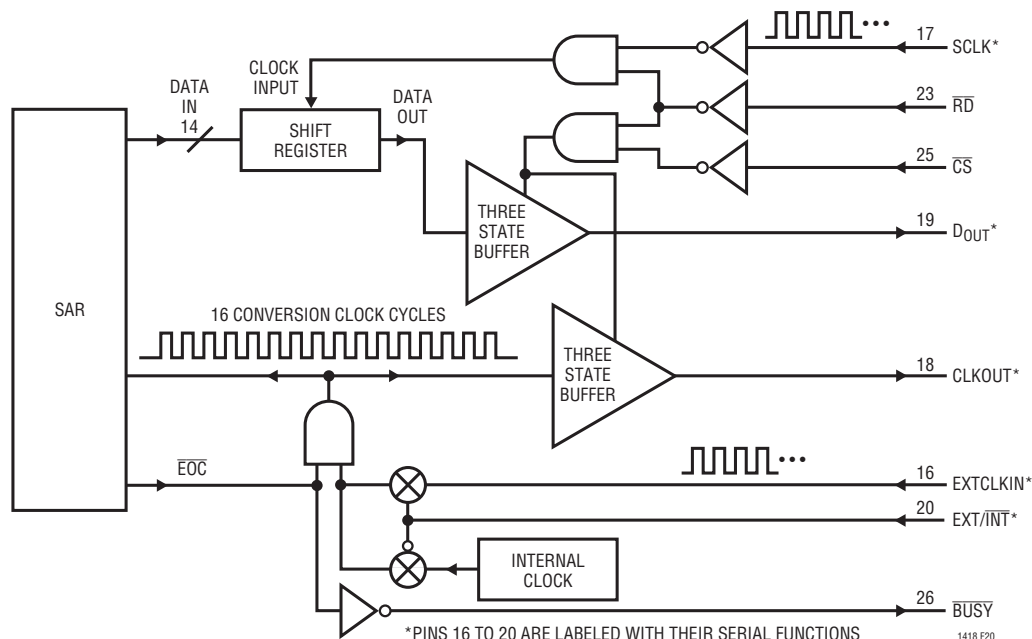
Figure 20. Functional Block Diagram for Serial Mode (SER/PA \overline{\text{R}} = High)
